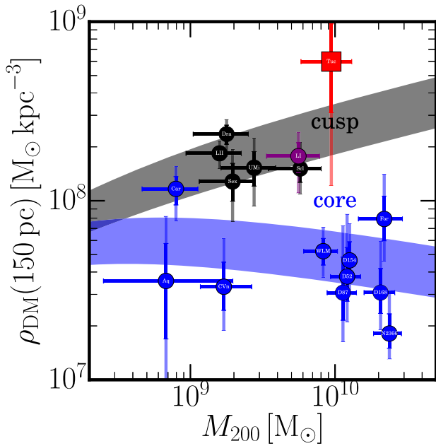
Figure 11. Inner DM density as a function of pre-infall halo mass for a selection of Local Group dwarf galaxies, as modelled in Read et al. (2018b). Black points shows galaxies whose star formation was truncated more than 6 Gyr ago; blue points show galaxies truncated less than 3 Gyr ago; and the purple points were truncated between 3 and 6 Gyr ago. The shaded regions highlight the expected DM density of cusped and cored profiles. Tucana is shown as the red point. In addition to highlighting the correlation between star formation history and the shape of the density profile, this plot shows the high central DM density of Tucana relative to other Local Group dwarf galaxies, a result which appears to be consistent with a central cusp.
