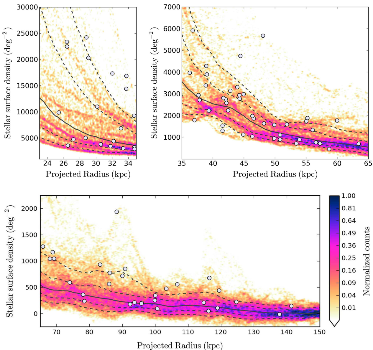
Figure 8. Distribution of surface density in the M31 halo for stars with -2.5 \lesssim [\text{Fe}/\text{H}] \lesssim -1.1 (i.e. ‘metal-poor’ stars), as a function of projected galactocentric radius within the PAndAS survey footprint. The full radial span has been split into three panels for clarity. Each panel has a different range on the y-axis, and the colour-map is normalized to the pixel with the highest number of counts; we use a non-linear (square-root) scaling to enhance the visibility of the tails of the distribution. The solid black contour shows the median of the distribution as a function of radius; the dashed contours show, from top to bottom, the 10 per cent, 25 per cent, 75 per cent, and 90 per cent bands (i.e. at any given radius the 10 per cent band has 10 per cent of the randomly generated locations sitting at higher surface density). Measurements for the 92 outer halo globular clusters are marked with light grey points.
