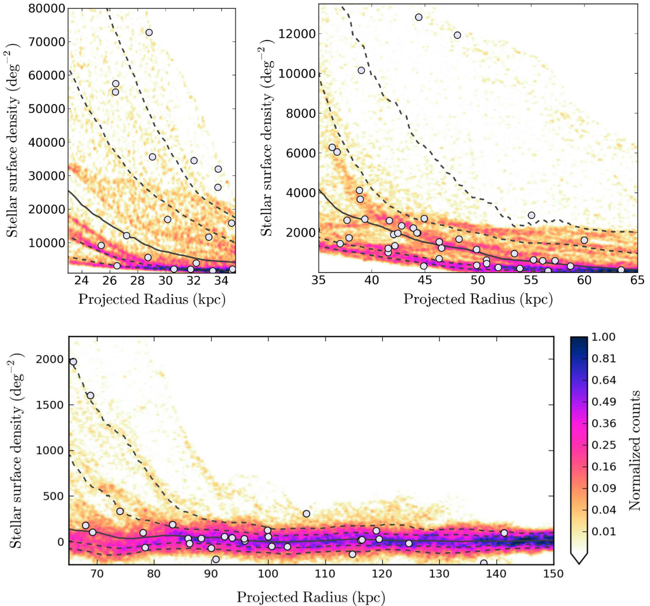
Figure 10. Same as Fig. 8, but now for M31 halo stars with -1.1 \lesssim [Fe/H] \lesssim 0.0 (i.e. ‘metal-rich’ stars). As before, the solid black contour shows the median of the distribution as a function of radius, while the dashed contours show, from top to bottom, the 10 per cent, 25 per cent, 75 per cent, and 90 per cent bands, and the measurements for our 92 outer halo globular clusters are marked with light grey points.
