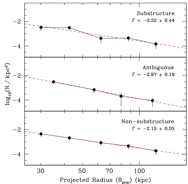
Figure 14. Radial surface density profiles for the three subgroups of outer halo globular cluster systems defined in Section 4.1. The red dashed lines show the best-fitting power-laws. All points have Poissonian error bars.
