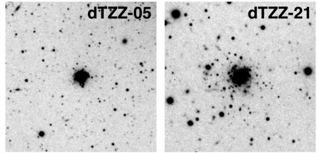
Figure 1. Gemini/GMOS images of the two confirmed outer halo globular clusters from the sample of di Tullio Zinn & Zinn (2015) that do not appear in Huxor et al. (2014). Each image is a 1' × 1' cut-out from a full GMOS i -band frame. North is to the top and east to the left.
