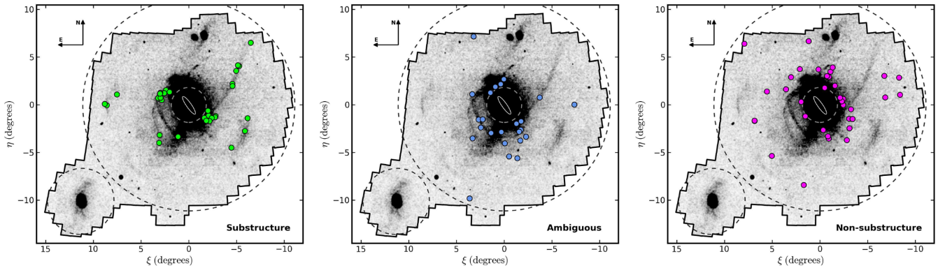
Figure 12. Spatial distribution for clusters in each of the three classes introduced in Section 4.1, overlotted on the metal-poor field halo map from Fig. 3.
