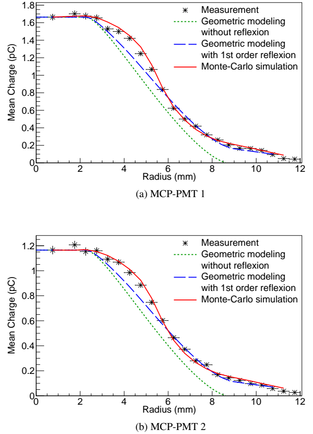
Figure 3: Radial distribution of the average signal charge for the two MCP-PMTs. Both MCP-PMTs are operated at 2800 V. The green dotted curve shows the expected distribution by geometrical calculation without including reflections. The blue dashed line shows the geometrical calculation after including first order reflections. The red line shows the distribution expected from a dedicated simulation that includes the detector characteristics (see text).
