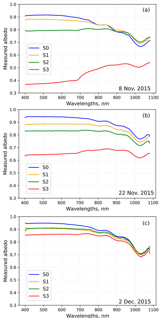
FIG. 4. Comparison of spectral albedo measured in Umiujaq on (a) 8 Nov, (b) 22 Nov, and (c) 2 Dec 2015 at four different sites (S0–S3). S0 is a lichen site with a pure snow surface, S1–S3 are shrub sites with shrubs of different heights: \sim 36 cm (S1), \sim 80 cm (S2), and \sim 120 cm (S3).
