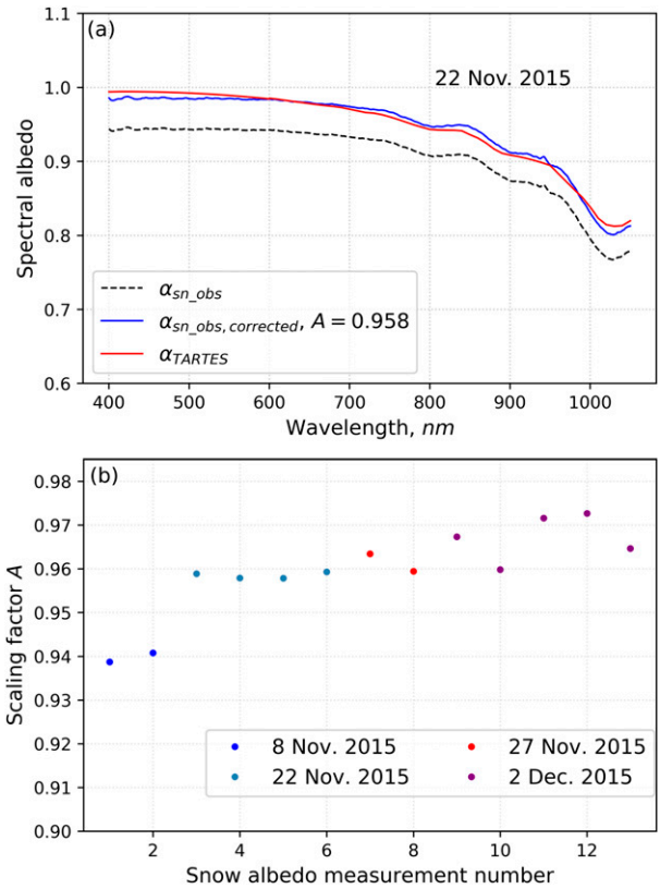
FIG. 7. Determination of the scaling factors used to correct artifacts in measured albedo. (a) \alpha_{sn\_obs} (black) is the spectral snow albedo measured at the lichen site S0 on 22 Nov. \alpha_{sn\_TARTES} (red) is the theoretical snow albedo computed with TARTES from the SSA profiles. \alpha_{sn\_obs,corrected} (blue) is the measured spectrum after correction with A = 0.958 . (b) Deduced scaling factors for all 13 snow albedo measurements taken at S0 during the autumn campaign 2015 in Umiujaq.
