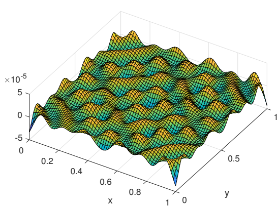
(a) 3D displacement field at 500.0 Hz.
