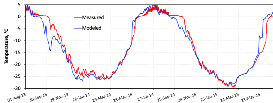
Figure 5. Measured and simulated ground temperature at 10-cm depth with Crocus.
