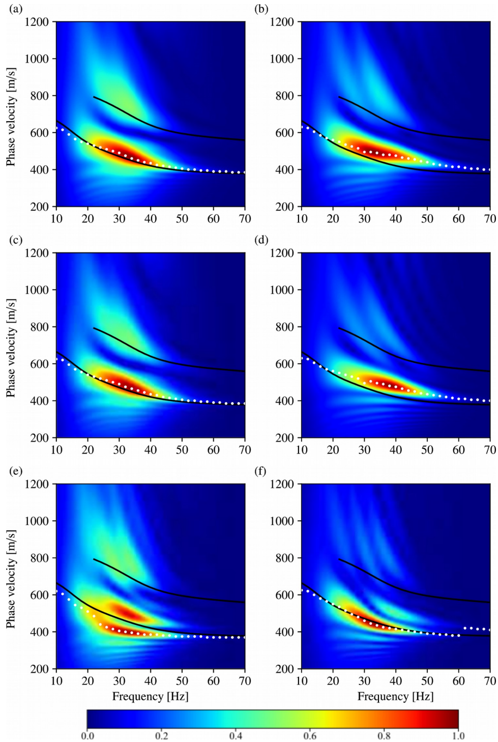
Figure 3: (a,b) Dispersion diagrams for the reference geometry model (a) without lateral variation of velocity ( V_{S3}=V_{S4}=400 m/s) and (b) with lateral variation of velocity ( V_{S3}=400 m/s, V_{S4}=500 m/s). (c,d) Same as (a) and (b) for the flat geometry models. (e,f) Same as (a) and (b) for the rough geometry models. Black lines correspond to theoretical fundamental and superior mode. White solid circles correspond to effective mode extracted from the dispersion diagram.
