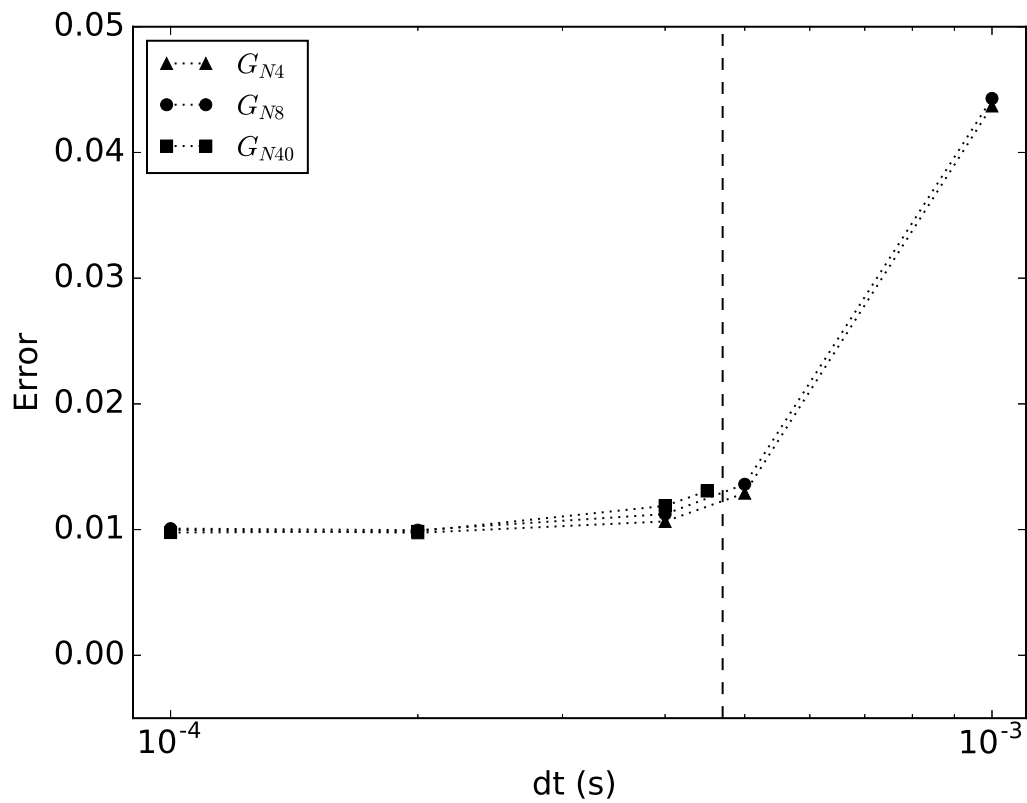
Figure 11: Error as a function of the time step dt with the optimal G(N) (in Figure 7). Three different degrees are displayed ( N = 4, 8 and 40 ). The optimal dt_c = 4.7 \times 10^{-4} s is displayed (dashed line). For N = 40 , the dt_{\text{CFL}} is reached before the optimal dt_c .
