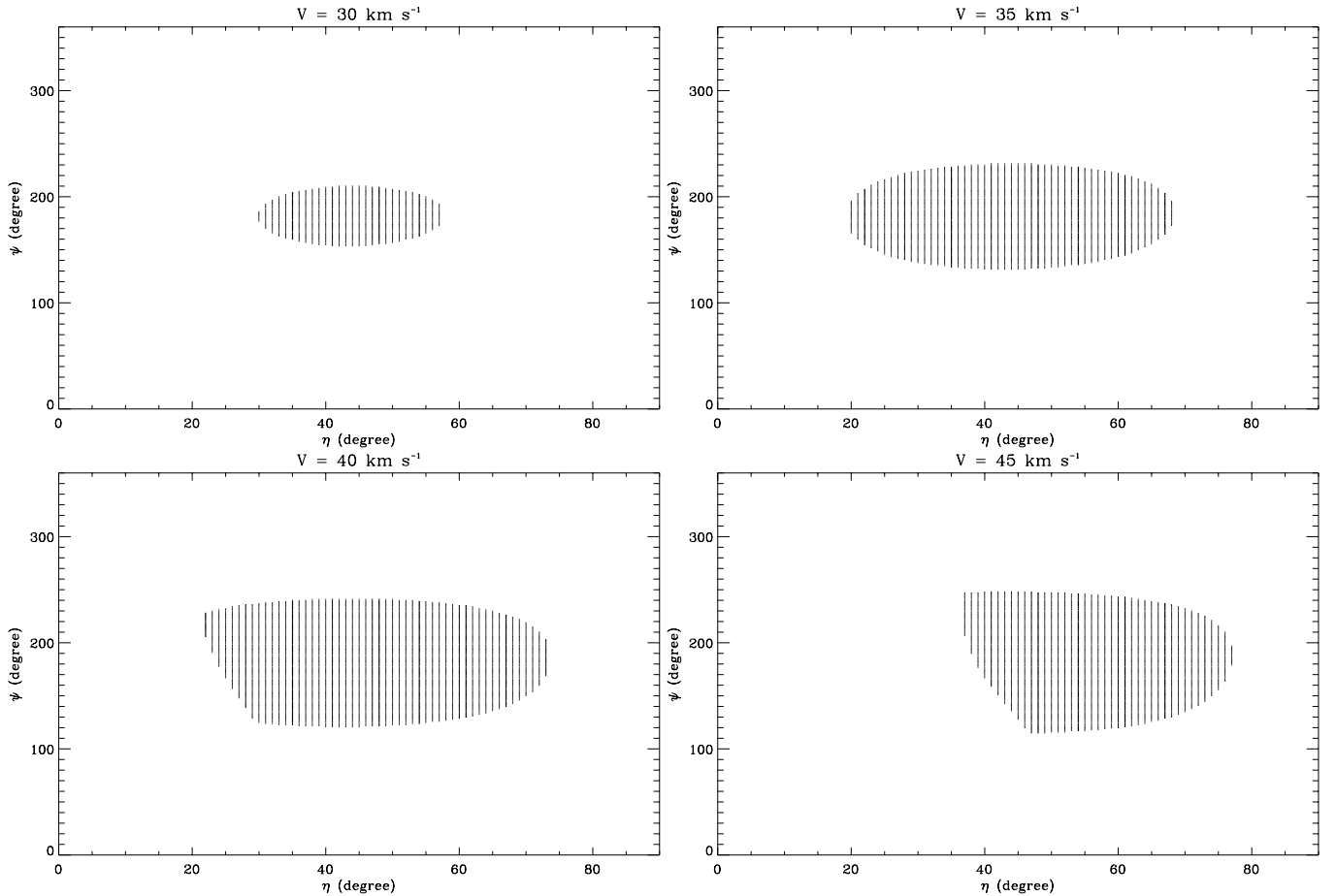
Fig. 11. (\eta, \psi) diagrams for velocity fields of 30, 35, 40 and 45 \text{km s}^{-1} . These diagrams give strengths and direction of velocity field vectors, which give results in agreement with the measurements. For a given value of the velocity field strength, only vectors with directions given by the shading area in the diagram give good results. According to these diagrams, if we limit ourselves to weakly inclined velocity fields ( 0^\circ < \eta < 20^\circ with respect to the polar axis ( Pz ) in Fig. 7), only velocity field with strengths between 35 and 39 \text{km s}^{-1} give polarization parameters and line ratio of the O vi doublet in consistence with the measured ones. If we take into account, in addition, velocity fields with mean inclinations ( 20^\circ < \eta < 30^\circ ), velocity fields with strengths between 30 and 43 \text{km s}^{-1} give good results. If we add highly inclined velocity fields ( 30^\circ < \eta < 45^\circ ), we obtain good results for velocity fields with strengths between 29 and 49 \text{km s}^{-1} . These results correspond to electronic density of 3.5 \times 10^6 \text{ cm}^{-3} . Electron densities greater than 4.0 \cdot 10^6 \text{ cm}^{-3} do not give results in agreement with the observations.
