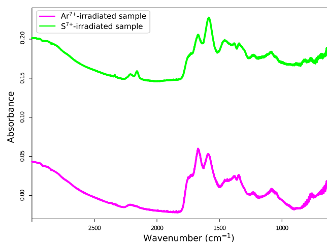
Figure 7. IR spectra of the residue, taken at 300 K, after irradiation by argon (Ar 7+ ions, magenta) and sulfur (S 7+ ions, green). The residue resulted from irradiated H 2 O:CH 3 OH:NH 3 ices (2:1:1).
