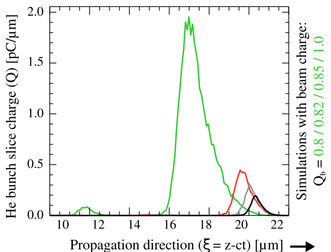
FIG. 6. Plot of the slice charge longitudinal density profile of the trailing beams injected via B-III near the back of the bubble at the end of the simulations, ct = 6 cm, performed with driver charges of 0.8, 0.82, 0.85, and 1 nC. Longitudinal axis corresponds to the comoving variable, \xi = z - ct , and the propagation direction is from left to right side of the plot.
