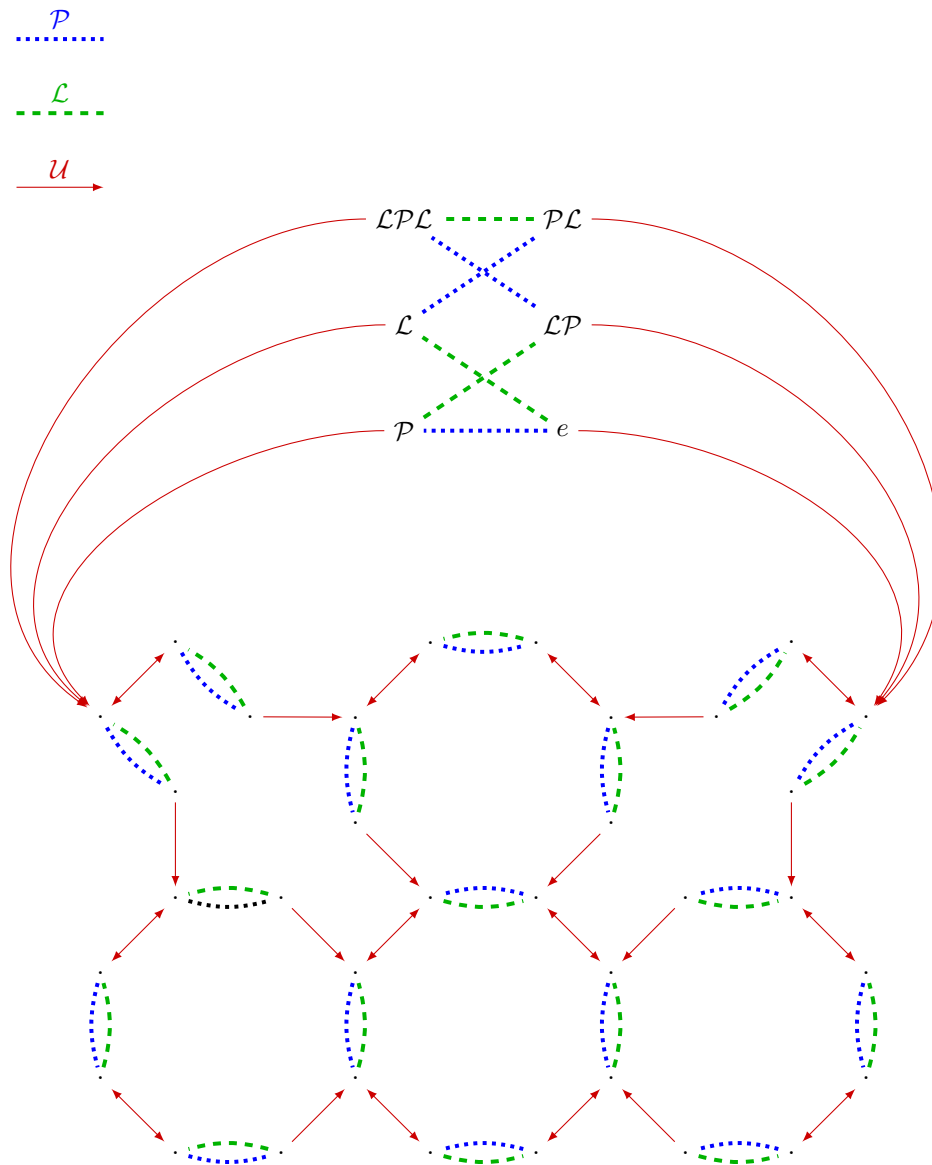
FIGURE 5. The Cayley graph of the monoid M_{U\mathcal{P}\mathcal{L}} generated by the relations U , \mathcal{P} , and \mathcal{L} . The relations \mathcal{L} and \mathcal{P} are involutions, and are represented as arrowless dashed and dotted lines.
