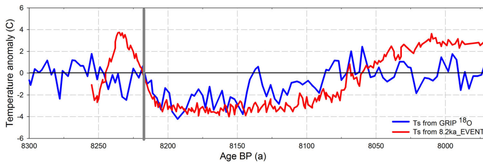
Figure 1. Time series of surface air temperature over central Greenland in 8.2ka_EVENT (red) compared to the GRIP temperature (blue) reconstruction from ice core \delta^{18}\text{O} (Thomas et al. , 2007). The vertical grey bar indicates the start of the 8.2 ka BP event climatic forcings input to LPJ-GUESS, which is the 31st year of the 8.2ka_EVENT simulation. [Color figure can be viewed at wileyonlinelibrary.com ].
