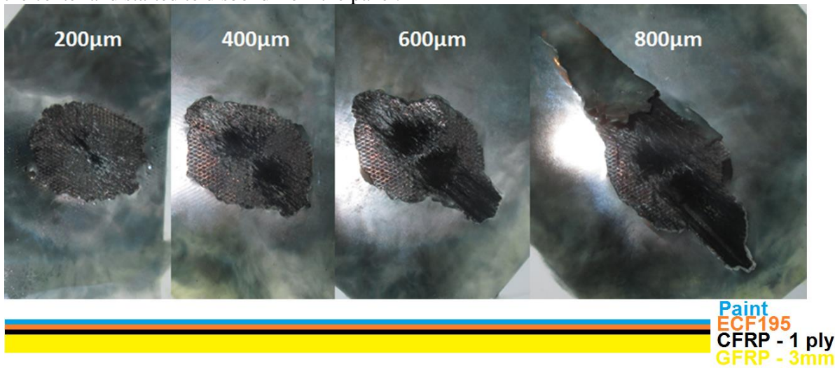
Figure 13 CFRP Current injection with paint thickness increase
