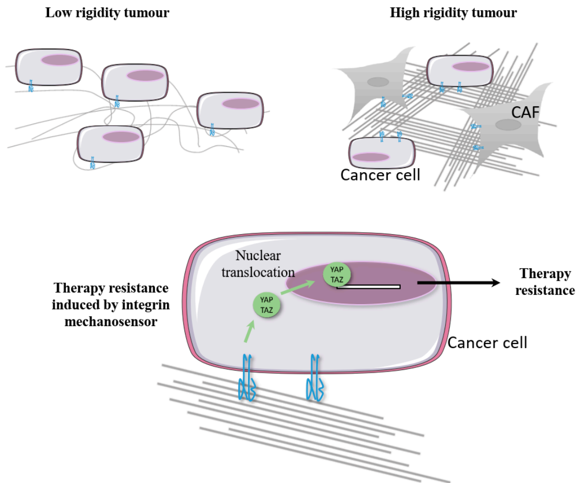
Figure 4. Hypothetic model showing how integrins may trigger therapy resistance in stiff micro-environmental niches. Therapy-resistant tumors are often characterized by an increase in matrix stiffness. Cancer-associated fibroblast (CAF) integrins (mainly \alpha 5\beta 1 integrin) generate mechanical forces that increase ECM protein assembly and matrix rigidity. In cancer cells, the sensing of CAF-generated tension by integrins activates transcriptional co-regulators YAP and TAZ and their translocation to the nucleus. The transcriptional response leads to therapy resistance (adapted from [186]).
