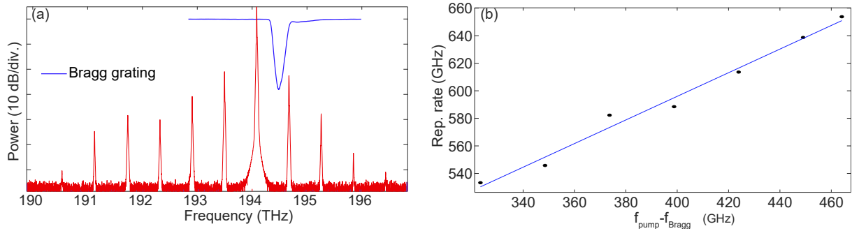
Fig. 1. (a) Output cavity spectrum (red curve) and fiber Bragg grating transmission curve (blue curve). (b) Comb repetition rate as a function of the pump to fiber Bragg grating frequency shift is plotted with black dots, the blue line is a linear fit.
