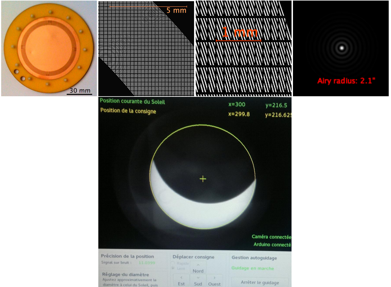
Fig. 4. Autoguiding images. Its objective lens is a ring-shaped Fresnel array ( top left ): a thin copper plate with several thousand subapertures. An image of the Sun is formed by diffraction and interference through the holes. Top center : two enlarged views of the Fresnel array holes. Top right : image of a monochromatic point source (point spread function) given by the Fresnel array. Bottom : control screen (photo by Géraldine Pedezert) of the autoguiding during the solar eclipse(2015-03-20). The solar disk is correctly located, even though only a crescent remains visible.
