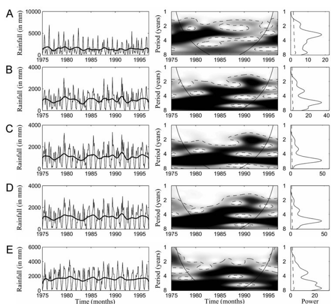
Figure 3 Wavelet analyses of the rainfall time series: (A) Cotiv021, (B) mean between GhanI32 and Ben270, (C) Ben270, (D) mean between Ben270 and Ben201, and (E) mean between Ben201 and Nige037. To deseasonalize the rainfall time series we removed all oscillating components with period less than 12 months using a low-pass Gaussian filter. In addition, all time series were normalized. For each time series, (i) the left panel displays rainfall time series. The solid and dense lines correspond to the raw time series and the deseasonalized time series, respectively. (ii) The middle panel shows the wavelet power spectrum for the different series (xaxis: time in year; yaxis: period in year). The power is coded from low values, in white, to high values, in black. The black dashed lines show the \alpha = 5\% significance level computed on 1,000 bootstrapped series. The inside area within the cone of influence (black line) indicates the region not influenced by edge effects. (iii) The right panel corresponds to the global wavelet spectrum (black line) with its significant threshold value of 5% (dashed line).
