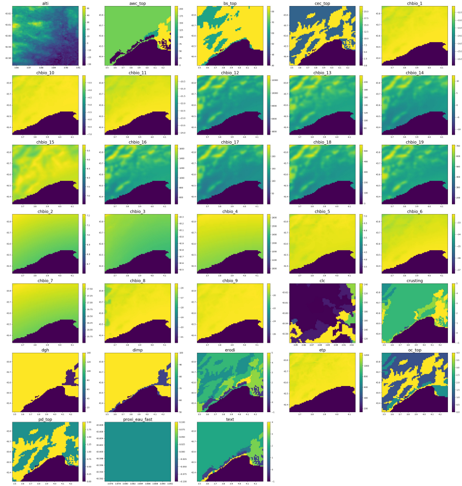
Fig. 1. Environmental rasters
