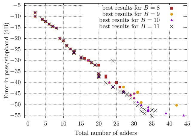
Fig. 8: Our designs with effective word lengths varying from 8 to 11, filter type I and smallest feasible filter order.
