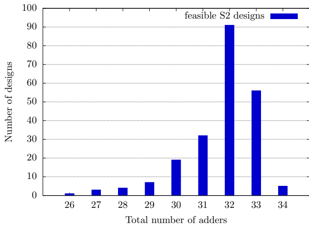
Fig. 4: Histogram demonstrating the total adder cost of feasible filter designs for S1 specification with word length B = 9 .
