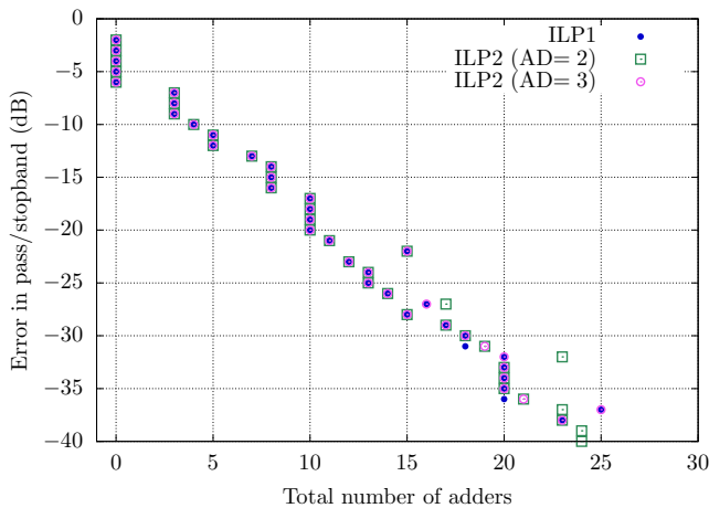
Fig. 7: Total adder count comparison when using ILP1 (adapted to minimize the total number of adders) and ILP2 (with AD limit set to 2) on the Redmill set of filters [4].
