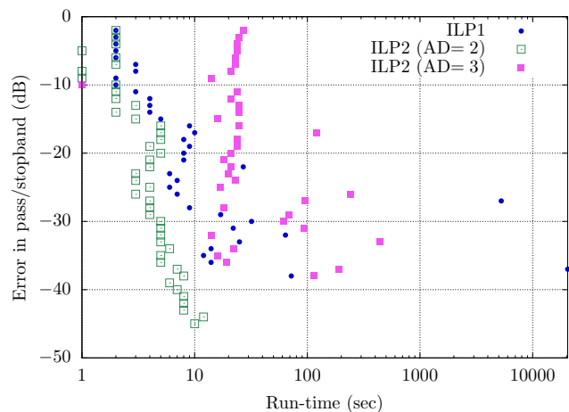
Fig. 6: Run-time for different pass/stopband errors for ILP1 and ILP2 with AD=2 and AD=3.
