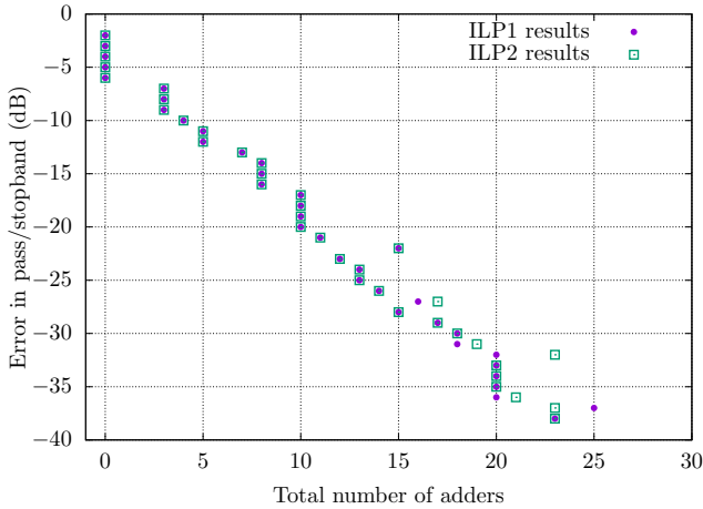
Fig. 6: Total adder count comparison when using ILP1 (adapted to minimize the total number of adders) and ILP2 (with AD limit set to 2) on the Redmill set of filters [4].
