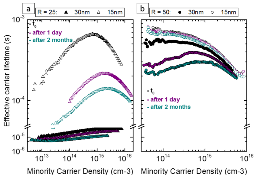
Figure 4. Effective carrier lifetime stability within time measured on symmetrical samples with poly-Si(B)/SiO x structure. The poly-Si(B) layer was developed using different gas flow ratio R during deposition: R = 25 (a) and R = 50 (b). For each ratio R , two poly-Si(B) thicknesses were targeted: 15 and 30 nm, resulting in different blister density (see Figure 1). PCD measurement was carried out after processing (black symbols), after 24 h (violet symbols) and 2 months (green symbols) of storage. The blister density was shown to play a role on surface passivation stability over time.
