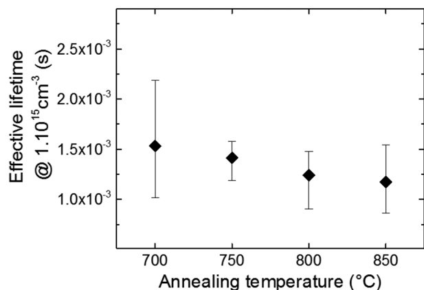
Figure 6. Monitor wafer lifetime variation when exposed to poly-Si(B) annealing thermal budget.
