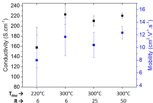
Figure 2. Lateral conductivity and free charge carrier mobility of the poly-Si(B) layer evaluated by Hall Effect technique after annealing at T_a = 700 °C ( d_{poly} = 30 nm). The deposition temperature T_{dep} and the gas flow ratio R = H_2/SiH_4 were tuned to reduce blistering of the poly-Si(B) layer after annealing which also reduced the measurement uncertainty of the lateral conductivity and mobility.
