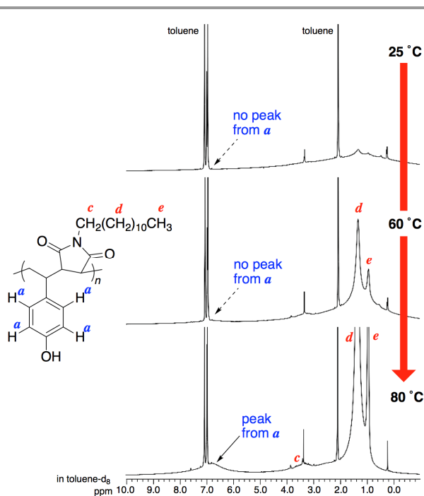
Fig 6. ^1\text{H} NMR spectra of 5wt% Alt-C12 gel in toluene- d_8 at 25 °C, 60 °C and 80 °C.
