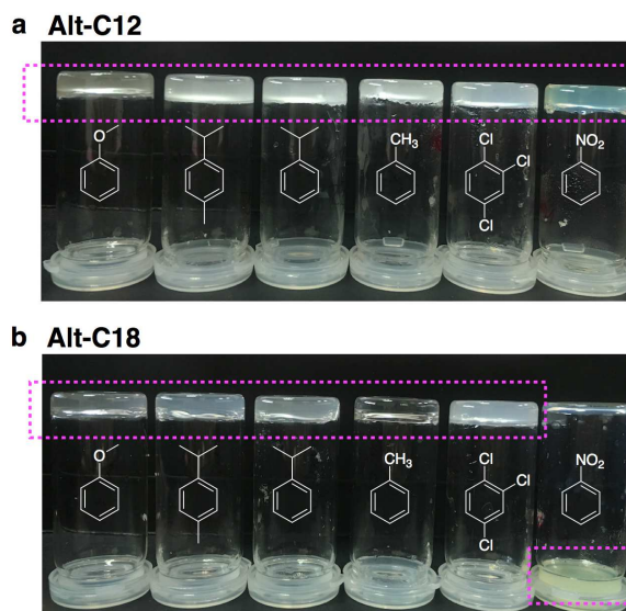
Fig 5. Appearances of 5wt% solutions of (a) Alt-C12 and (b) Alt-C18 in various aromatic solvents at ambient temperature (~25 °C) after cooling from 80 °C. The sample tubes were turned upside down for demonstration of gel formation (from left to right: anisole, p -cymene, cumene, toluene, 1,2,4-trichlorobenzene, nitrobenzene solvents).
