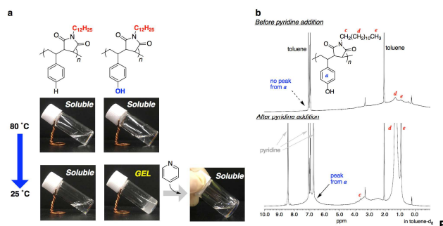
Fig 7. (a) Relation between polymer structures and solubilities and (b) ^1\text{H} NMR spectra of 5wt% Alt-C12 gel in toluene- d_8 (upper) and after addition of pyridine (lower): [phenol unit in gel] = [added pyridine].
