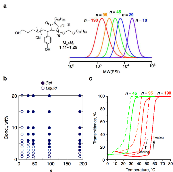
Fig 8. (a) GPC curves of copolymers synthesized by RAFT polymerization and deprotection reaction: [tBOS]_0/[C12MI]_0/[CTA]_0/[AIBN]_0 = 1000/1000/5/1 mM ( n = 190 ), 1000/1000/10/1 mM ( n = 95 ), 500/500/10/1 mM ( n = 45 ), 300/300/10/1 mM ( n = 29 ), 100/100/10/1 mM ( n = 10 ) in toluene at 60^\circ\text{C} , (b) polymerization degree ( n )–concentration plot: (filled circle: gel, open circle: liquid) and (c) turbidity measurements for 1wt% copolymer solutions in toluene ( n = 45, 95, 190 ) (heating speed = 0.5^\circ\text{C}/\text{min} , wavelength \lambda = 670 nm).
