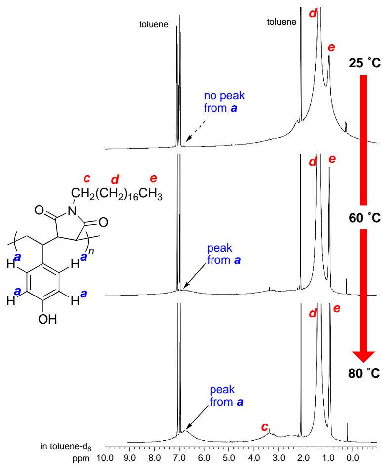
Figure S7. ^1\text{H} NMR spectra of 5wt% Alt-C18 gel in toluene- d_8 at 25 °C, 60 °C and 80 °C.
