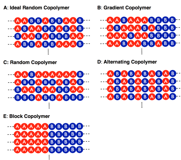
Fig. 1 Various copolymers: (A) ideal random copolymer; (B) gradient copolymer (C) random copolymer of broad composition distribution; (D) alternating copolymer; (E) block copolymer.
