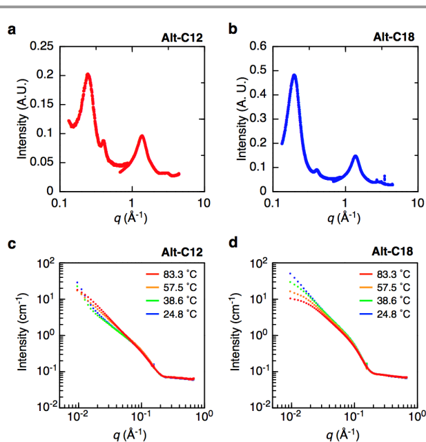
Fig 10. Wide angle X-ray diffraction patterns of freeze dried bulk Alt-C12 (a) and Alt-C18 (b) (The peak arising at q = 0.4 \text{ \AA}^{-1} ( 2\theta = 2.7^\circ ) is due to Kapton windows.) and SANS profiles of 5wt% Alt-C12 (c) and Alt-C18 (d) in toluene-d 8 at various temperatures.
