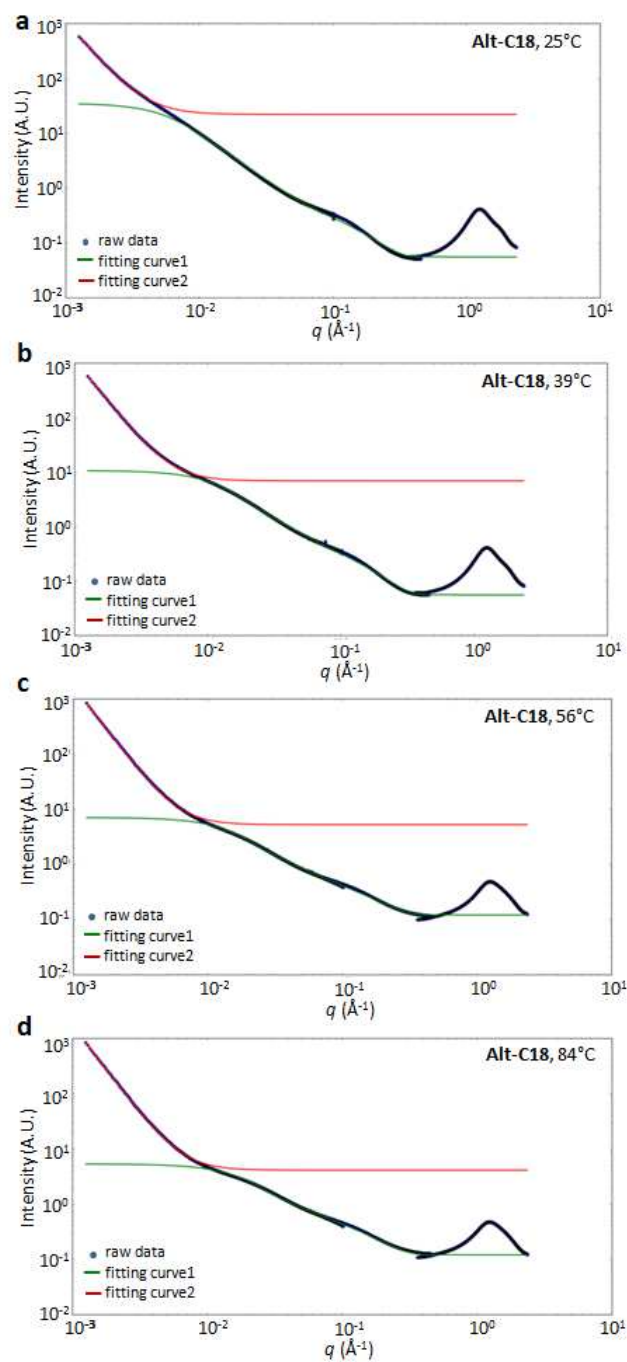
Figure S12. SAXS data with fitting curves for Alt-C18 (a-d) at different temperatures. The fitting curve1 (green) correspond to a flexible cylinder model fitted from 0.01 to 0.5 \text{ \AA}^{-1} . The fitting curve2 (red) correspond to a shape unique power law model fitted from 0.001 to 0.01 \text{ \AA}^{-1} .
