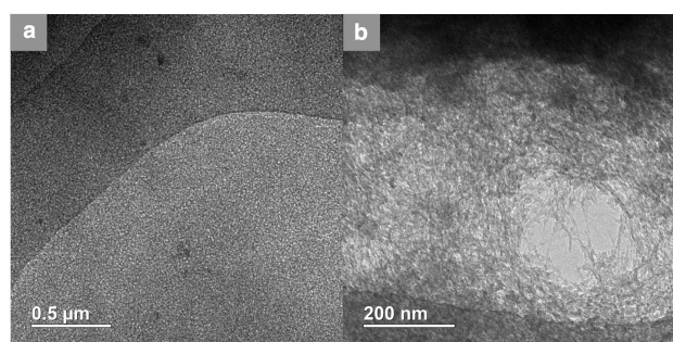
Fig 11. Cryo-TEM images of Alt-C18 at 5wt% in cumene. The left picture (a) is taken at the edge of the carbon grid. In the right picture (b), the fibrillar morphology is revealed inside a tear defect.
