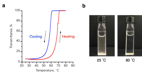
Fig 4. (a) Turbidity measurement of 1wt% Alt-C12 solution in toluene: heating speed = 0.5 °C/min, wavelength \lambda = 670 nm, (b) pictures of the 1wt% Alt-C12 solution in toluene at 25 °C and 80 °C.
