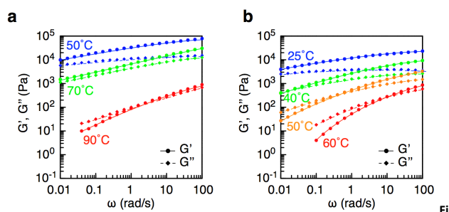
Fig 9. Rheology of organogels 10wt% in 1,2,4-trichlorobenzene ( \gamma=1 ): (a) Alt-C12 and (b) Alt-C18 .
