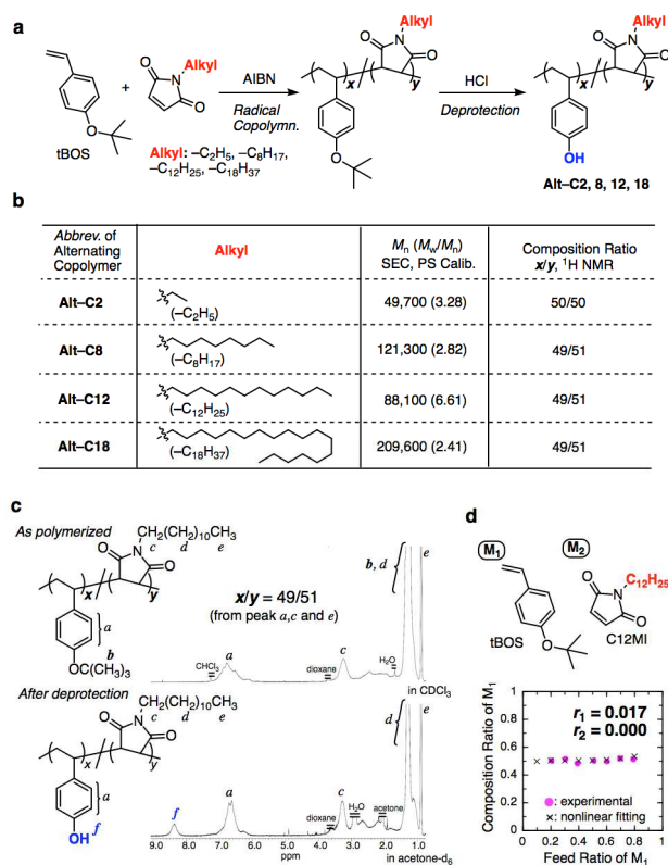
Fig. 3 (a) Synthetic scheme of alternating copolymers with 4-vinylphenol and N -alkylmaleimide: [tBOS] _0 /[ N -alkylmaleimide] _0 /[AIBN] _0 = 1000/1000/20 mM in toluene at 60^\circ\text{C} , (b) table of molecular weight and composition of copolymers after deprotection reaction, (c) ^1\text{H} NMR spectra of the copolymer with tBOS and C12MI (upper) and the copolymer after deprotection reaction (lower) and (d) monomer reactivity ratios of tBOS ( M_1 ) and C12MI ( M_2 ) calculated from non-linear fitting method.
