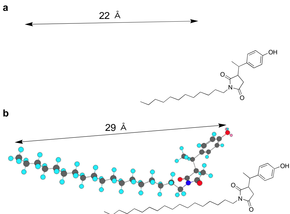
Figure S9. Chem3D Molecular models of dimers of 4-vinylphenol and N -alkylmaleimide (a, C12MI; b, C18MI) with alkyl chains in the fully extended conformation.
