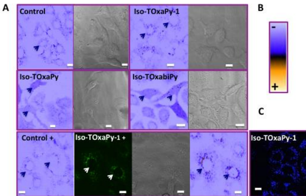
Figure 8. Detection of the compounds by their intrinsic fluorescence. A) HeLa cells treated for 17 h, in the presence of the compounds (2 \mu\text{M} for iso-TOxaPy and iso-TOxabiPy, and 3.3 \mu\text{M} for iso-TOxaPy-1) are imaged, with excitation wavelength at 488 nm, in the absence of any additional fluorophore. For a better visualization, the green signals are turned to a rainbow false color (scale shown in B). The corresponding wide fields allow visualizing the nucleus and the cell border. [iso-TOxaPy-1 +] and [control +] indicate that the power laser was increased compared to upper images. The bright field and the green signal correspond to the iso-TOxaPy-1+ treatment. Arrows point to nucleus. B) Rainbow blue to orange scale used to better visualizing the fluorescence in B. C) The cells treated with iso-TOxaPy-1 (3.3 \mu\text{M} ) were imaged following a 405 nm excitation. In B and C, the bar represents 10 \mu\text{m} .
