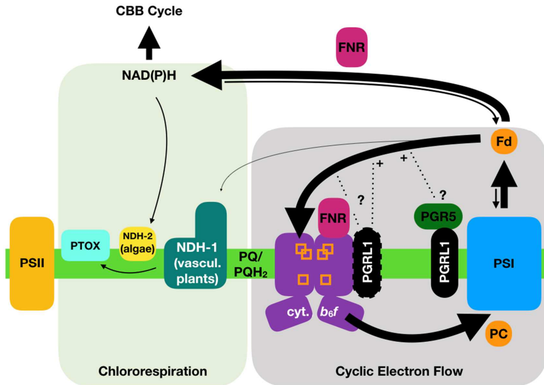
Fig. 1. A scheme of CEF and chlororespiration, and the molecular actors involved in these processes. PGRL1 (dashed) could almost stoichiometrically bind to cyt. b_6f to regulate CEF. Note that chlororespiration rates are so low that the only contribution of this process is observed in darkness [16].
