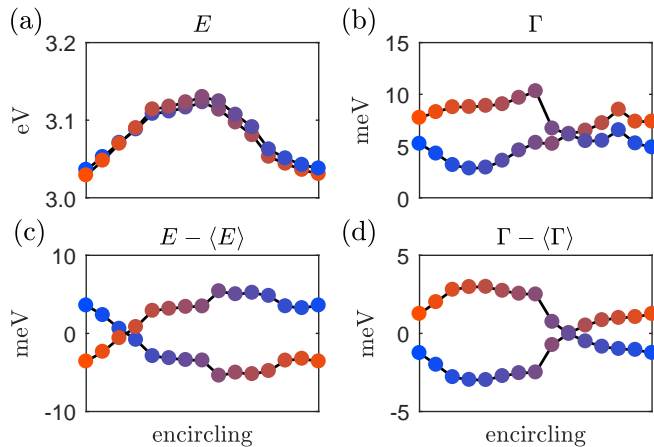
FIG. 4. Clockwise encircling of a Voigt point in \vec{k}_{\parallel} space along the trajectory shown in Fig. 1 (b) with the same color code. (a): mode energies degenerate near the fourth point; (b): mode broadenings degenerate near the twelfth. Encircling once flips one mode to the other, encircling twice yields the initial situation (complex-square-root topology). For better visibility, the mean values are subtracted in (c,d). See further trajectories in the SM [33].
