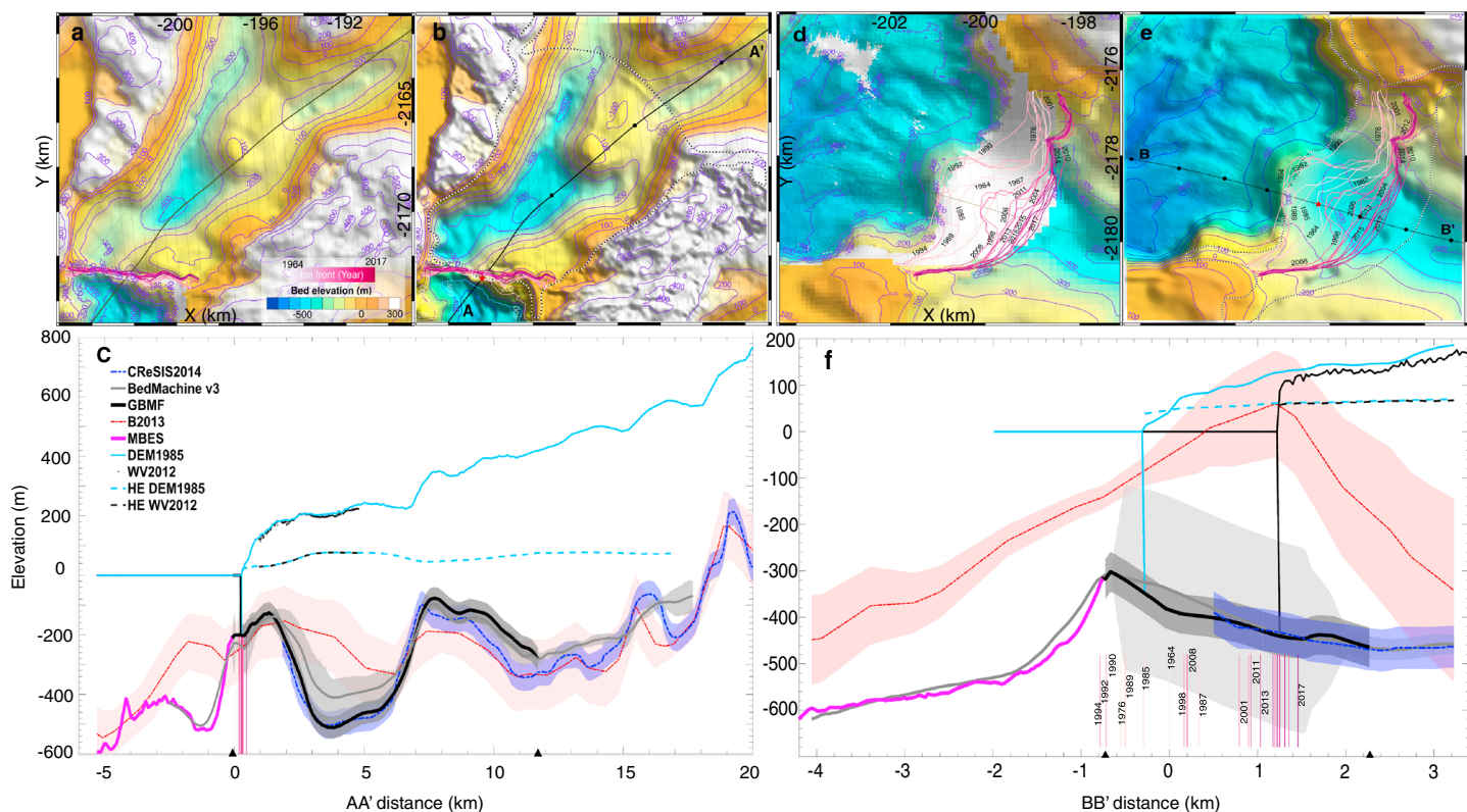
Figure 2. (a and d) Mass conservation bed elevation on land and multibeam echo sounding (MBES) in the ocean for Sermeq Avannarleq and Kujalleq, Greenland. (b and e) Bed elevation from gravity color coded from white to orange (300 m to 0 m) to green, blue, and dark blue (100 to 800 m depth) with 100 m contours in purple. Profile AA' and BB' are CReSIS RES data from 14 April 2014 and 6 April 2013, respectively (Figure S4). Black circles indicate 5 km intervals from the 1964 ice front (red star) of Sermeq Avannarleq and 1 km intervals for Kujalleq. (c and f) Glacier surface and bed elevation from this study are thick black lines with errors in dark gray, BM3 (Morlighem et al., 2017) is light gray, CReSIS is blue, Bamber et al. (2013) is red, and MBES is magenta. Black triangles indicate the limits of the gravity inversion.
