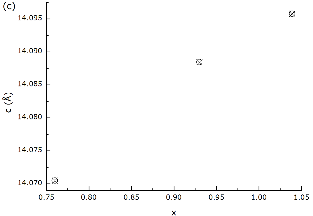
Figure 3: (a) and (b) lattice parameters as a function of temperature measured by powder XRD ; (c) relation between the c lattice parameter and the x value.
