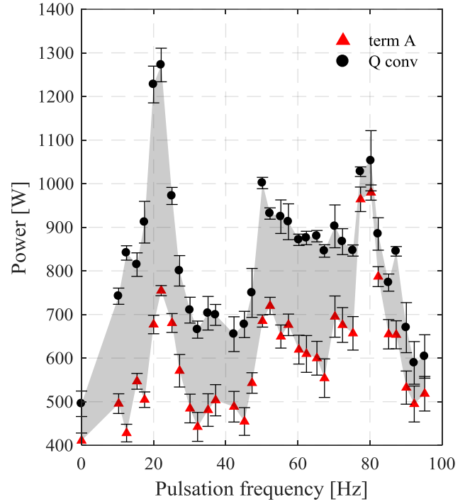
Figure 6: Energy balance equation terms, w/ dry ice, L = 5.91\text{m}
