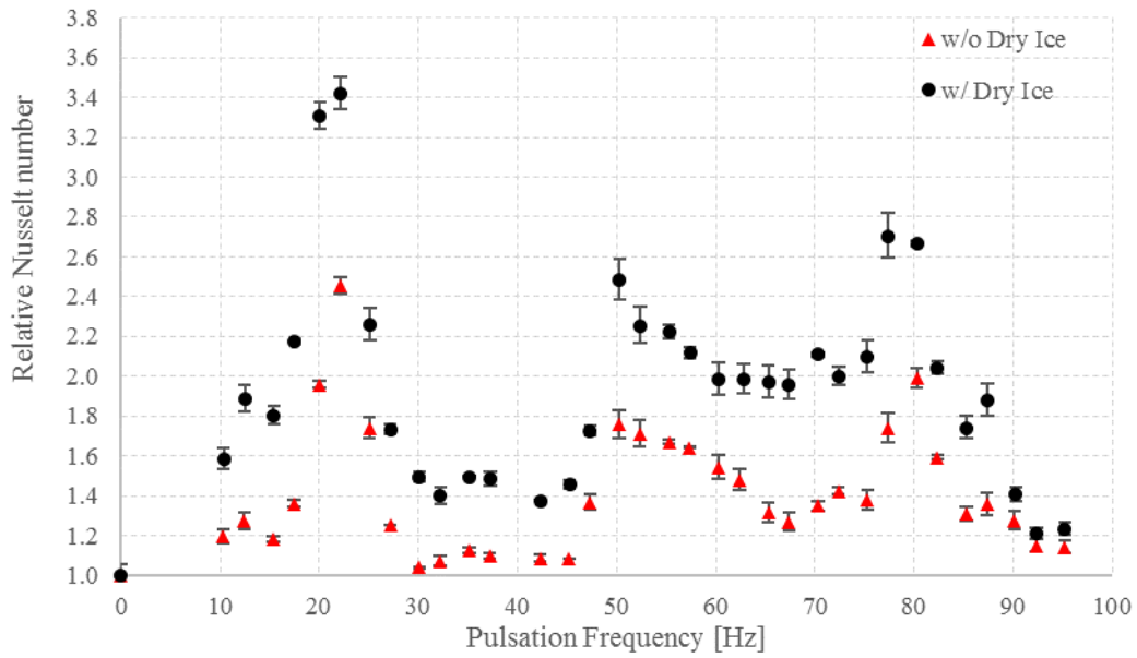
Figure 7: Relative time-averaged Nusselt number, L = 5.91m
