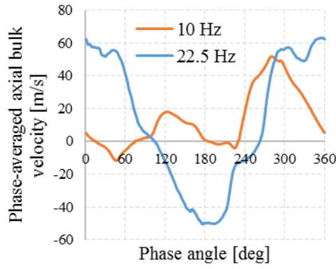
Figure 8: Axial component of the phase-averaged bulk air velocity, axial position B-B', L = 5.91\text{m} , Re = 30000
