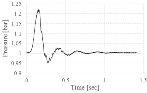
Figure 3: Instantaneous pressure, L = 5.91\text{m}
