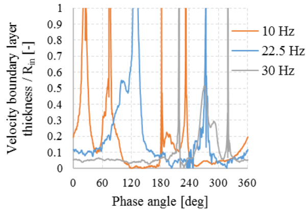
Figure 12: Velocity boundary layer thickness on the pipe internal radius, axial position B-B' , L = 5.91m , Re = 30000
