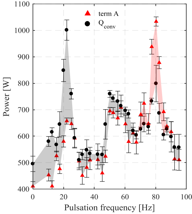
Figure 5: Energy balance equation terms, w/o dry ice, L = 5.91\text{m}
