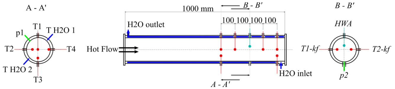
Figure 2: Test-section
