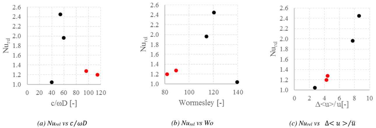
Figure 13: Relative time-averaged Nusselt number as a function of dimensionless parameters
