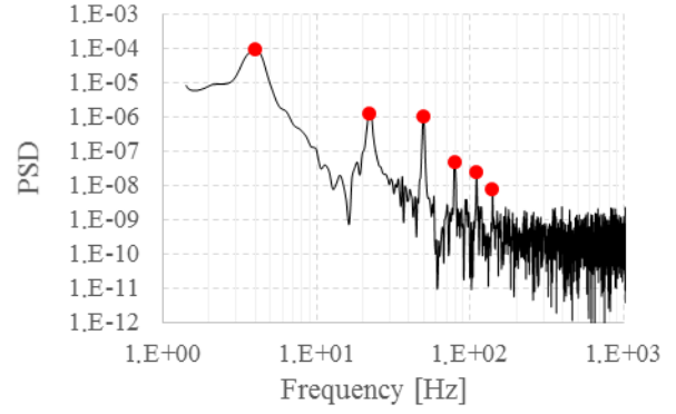
Figure 4: Power Spectral Density, L = 5.91\text{m}
