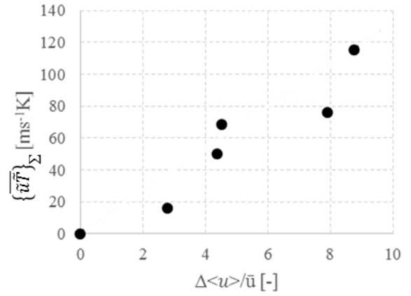
Figure 11: \{\bar{u}\tilde{T}\}_\Sigma as a function of \Delta\langle u \rangle / \bar{u}
