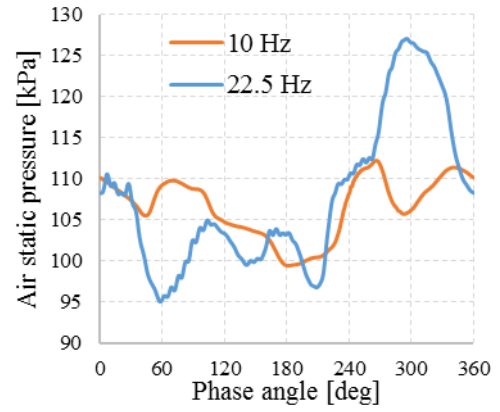
Figure 9: Phase-averaged air static pressure, axial position B-B', L = 5.91\text{m} , Re = 30000
