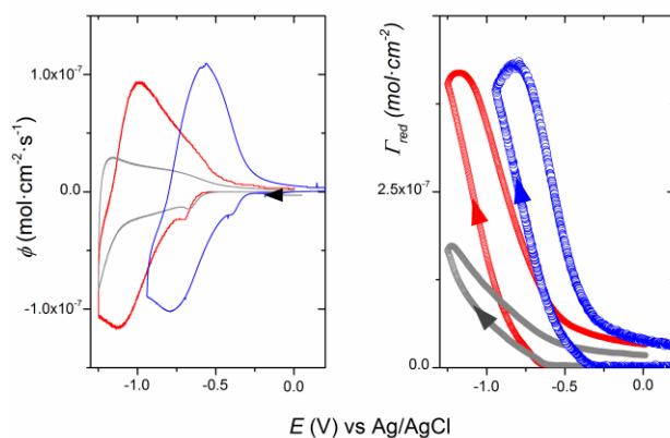
Figure 2. (Left) CVs and (right) CVAs (monitored at 780 nm) recorded simultaneously at a 1 \mu m-thick GLAD-TiO 2 electrode in an aqueous solution of (blue) 14 mM HCl (pH 1.85), or buffered solutions (pH 7.0) of (black) 1 mM HEPES or (red) 100 mM HEPES. All solutions also contained 0.3 M KCl as supporting electrolyte. Electrodes were scanned from 0 to -1.25 V at pH 7, and from 0 to -0.96 V at pH 1.85. CVs are expressed in flux density and CVAs in surface concentrations (i.e., \Delta A_{780}/(1000 \cdot \epsilon_{780}) ). Scan rate: 0.1 V·s -1 . T = 25^\circ\text{C} .
