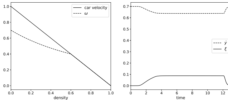
Figure 1: Evolution in time of the subjective density \xi and the bus velocity \dot{y} (1280 cells).
