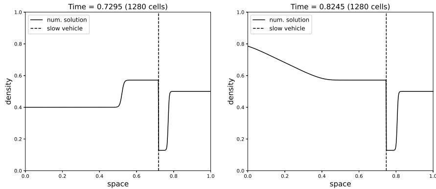
Figure 4: Evolution in time of the numerical density corresponding to initial data (5.1) (left) and (5.2) (right), with 1280 cells.
