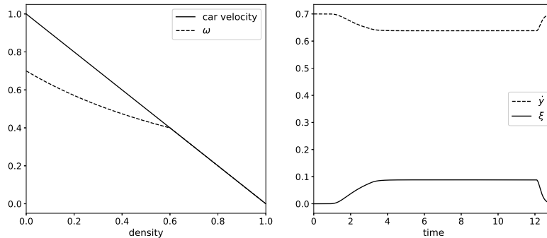
Figure 1: Evolution in time of the subjective density \xi and the bus velocity \dot{y} (1280 cells).
