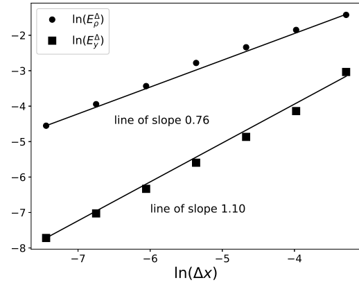
Figure 3: Rates of convergence at time T = 13 .
