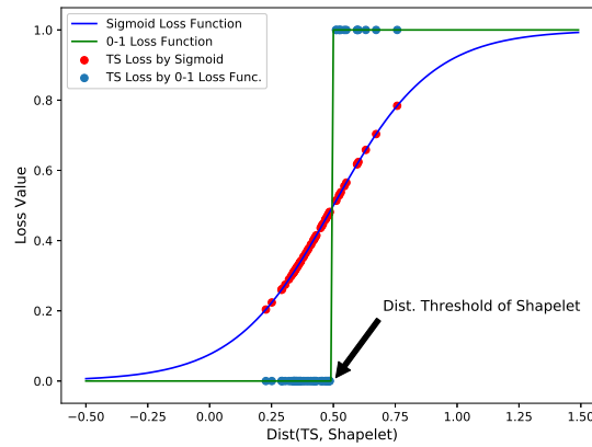
Figure 3: Loss measure of Time Series by Sigmoid Function and 0-1 Loss Function, Time Series in different classes are distributed around the split point of Shapelet
