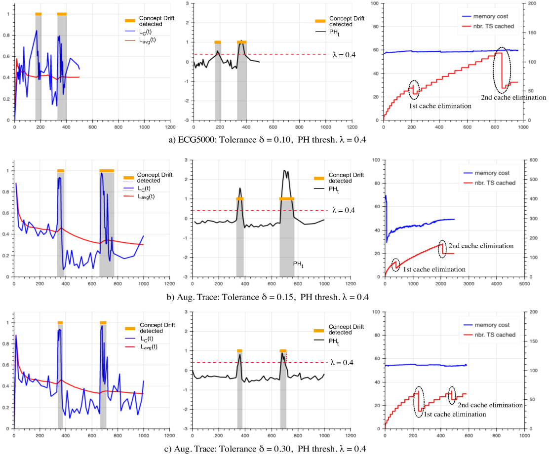
Figure 7: Results of Concept Drift Detection on ECG5000 dataset and augmented Trace dataset
