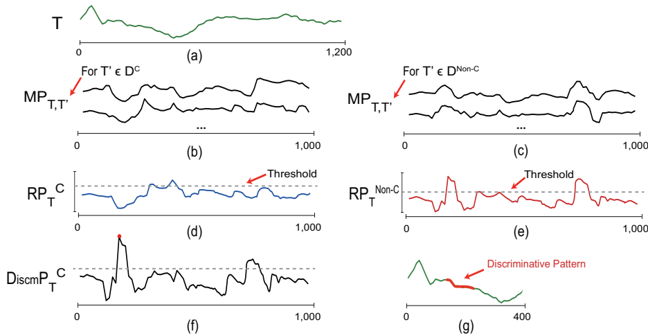
Figure 2: (a) Time Series T with class C . (b,c) Matrix Profile set for T with TS instances in different classes. (d,e) Representative Profile of T in different classes. A threshold can determine the representative area in T . (f) Discriminative Profile of T in dataset. The highest point in DiscmP_T^C identifies the most discriminative pattern's in T .
