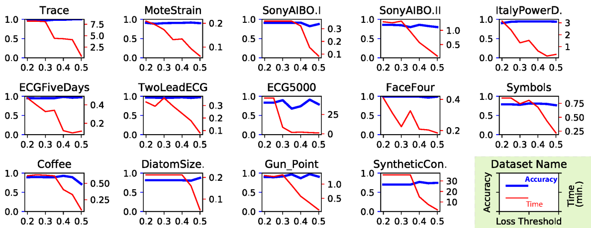
Figure 6: Results of Incremental Test (ISMAP) by adopting an extra Shapelet Evaluation procedure
