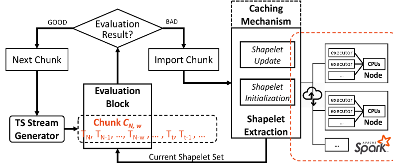
Figure 4: System Structure in TS Stream context with Concept Drift
