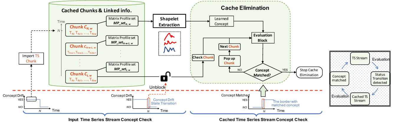
Figure 5: Elastic Caching Mechanism for streaming instance chunk in memory
