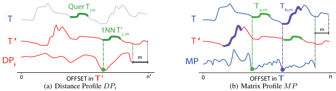
Figure 1: (a) Distance Profile between Query T_{i,m} and target time series T' , where n' is the length of T' . Obviously, DP_{i,j} can be considered as a meta TS annotating target T' ; (b) Matrix Profile between Source time series T and Target time series T' , where n is the length of T . Intuitively, MP_i shares the same offset as source T
