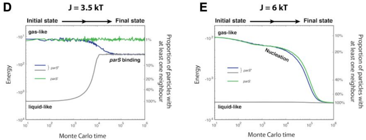
S3D-E Monte-Carlo simulations of the Lattice-Gas model for weak (left panel) and strong (right panel) interaction strengths between ParB particles. (D) Weak ParB-ParB interactions ( J=3.5 \text{ kT} ) and high-affinity ParB-parS interactions are considered here. Regardless of initial conditions (gas or liquid-like state), ParB proteins are unable to form a condensate in the presence of parS10 (gray, blue) and the system equilibrates to a state where only ParBs bind specifically to the centromeric sequences. (E) In contrast, when strong ParB-ParB interactions ( J=6 \text{ kT} ) are considered, small droplets immediately appear and nucleate into a single larger condensate independently of the presence or absence of a nucleation sequence (blue and green curves, respectively).
