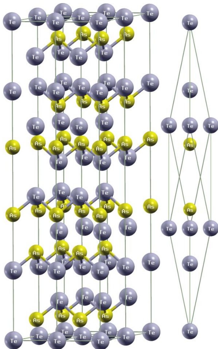
Fig. 1. Tetradymite crystal structure of \beta -As 2 Te 3 : hexagonal unit cell (left) and rhombohedral primitive cell (right).
