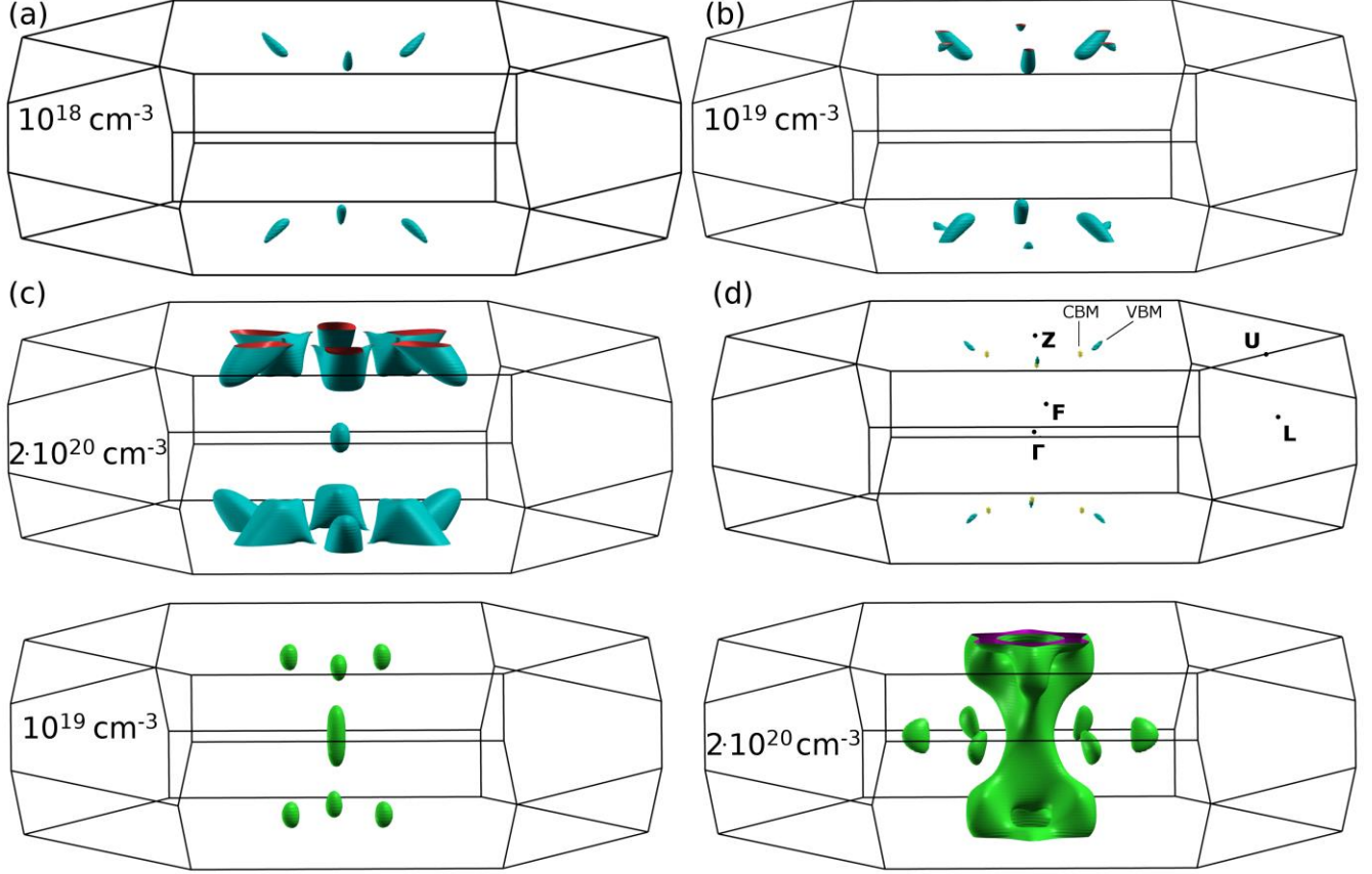
Fig. 5. Fermi surface (FS) of p - and n -type \beta\text{-As}_2\text{Te}_3 computed for carrier concentrations: (a) p = 10^{18} \text{ cm}^{-3} , (b) p = 10^{19} \text{ cm}^{-3} , (c) p = 2 \times 10^{20} \text{ cm}^{-3} , (e) n = 10^{19} \text{ cm}^{-3} , (f) n = 2 \times 10^{20} \text{ cm}^{-3} . In panel (d), the isoenergetical surfaces for the conduction (valence) band at 2 meV above (below) band edges are plotted to better visualize the indirect structure of the band gap.
