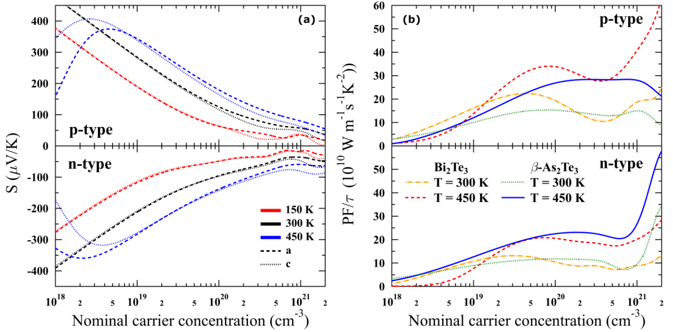
Fig. 8. (a) Thermopower of p - and n -type \beta\text{-As}_2\text{Te}_3 along the binary ( a ) and trigonal ( c ) axis calculated at three selected temperatures. In agreement with experimental results, the anisotropy is very small. (b) Average power factor (PF) divided by the scattering time \tau for \beta\text{-As}_2\text{Te}_3 . For comparison purposes, the results are compared to those obtained for \text{Bi}_2\text{Te}_3 .
