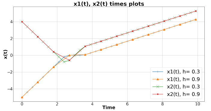
Fig. 6. Time plots of the solutions x_1(t) and x_2(t) for B = (-0.5, 1) and h = 0.9 or h = 0.3 . Initial condition is \mathbf{x}_0 = (-5, 4)
