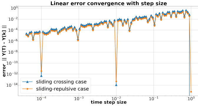
Fig. 7. Error \|Y(t) - Y_k\| with respect to time step h . We consider the two kind of AC solutions: the sliding-crossing solutions and the sliding-repulsive solutions.
