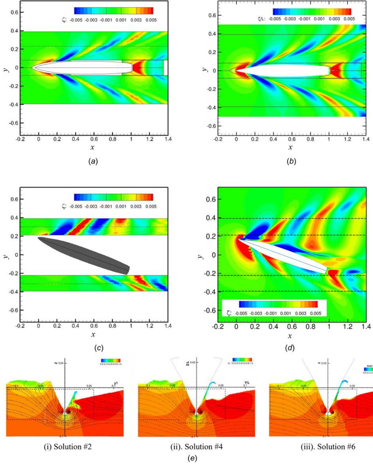
Fig. 2 Wave-elevation contours obtained using: (a) experiment and (b) S3 for \beta = 0^\circ ; (c) experiment and (d) S4 for \beta = 20^\circ . (e) Wave elevation pattern predicted by solution #2 (using level set) and S4 and S6 (both using VoF) at x = 0.1 shows the differences in wave breaking pattern on the leeward sonar dome.
