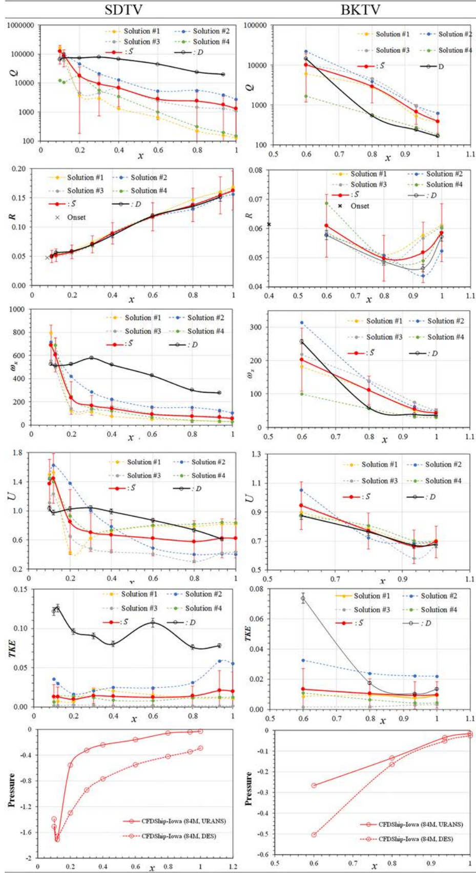
Fig. 9 Axial variation of flow variables in SDTV (left column) and BKT (right column) cores obtained using S1 through S4, and mean code with P_{E1} bars is compared with experimental data with U_D bars for \beta = 20 deg. The SDTV onset at x = 0.077 and BKT onset at x = 0.4 are shown in radial location ( R ) subplot.
