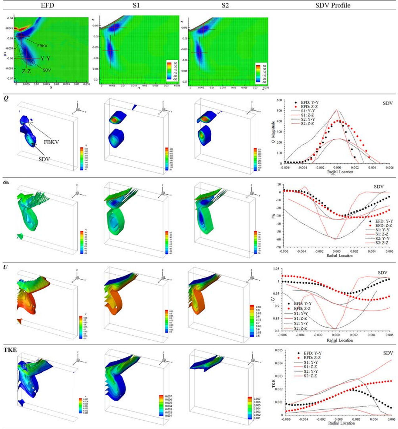
Fig. 6 Cross plane vortex core predictions for \beta = 0 deg at x = 0.2 . (Top row) Contour of axial vorticity, contour lines of Q , grid lines, and cross-plane analysis Y-Y and Z-Z lines. Volume plots showing 3D structures of the SDV and FBKV flow variables obtained the experimental data (left), S1 (2nd column) and S2 (3rd column). Subplots on the (right) are compared with y -y and z -z profiles of the flow variables in the SDV core predicted by S1 and S2 with the experimental data. For y -y line, the -y radial location is toward the center plane. For z -z line, the -z radial location is away from the hull.
