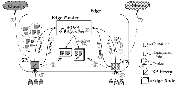
Figure 1: Architecture of MORA .
