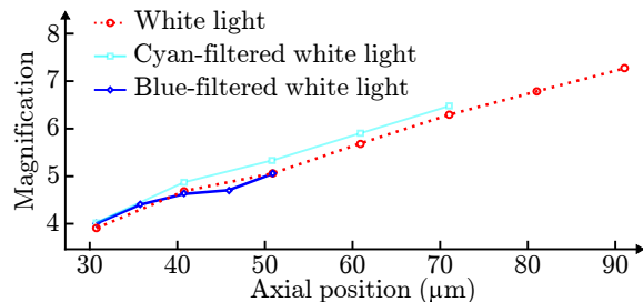
Figure 4: Evolution of the lateral magnification from a 25- \mu\text{m} -diameter microsphere placed in air as a function of axial position under three types of light source having 400 nm (in red line), 90 nm (in cyan line) and 11 nm (in blue line) of bandwidth.
