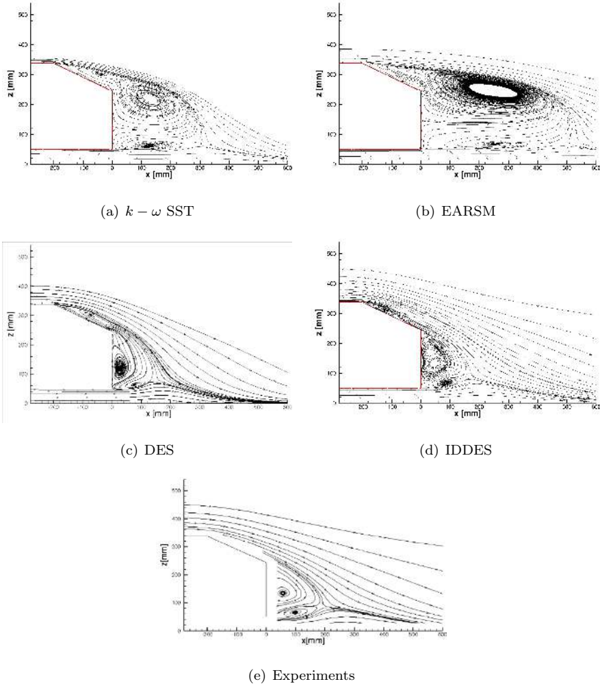
Figure 17: 25^\circ slant angle - Streamlines in the symmetry plane Y = 0 .
