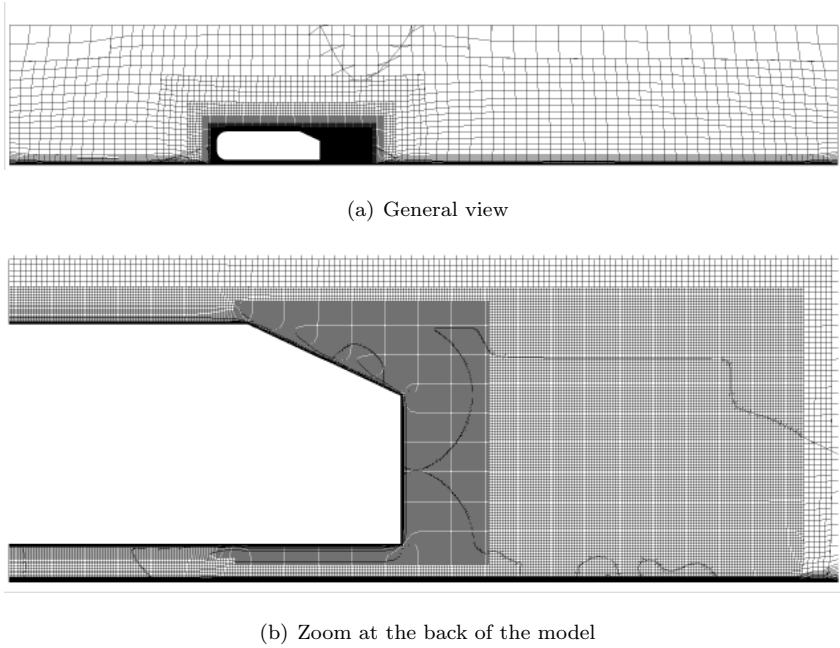
Figure 2: View of the mesh in the symmetry plane for the 25^\circ slant angle.
