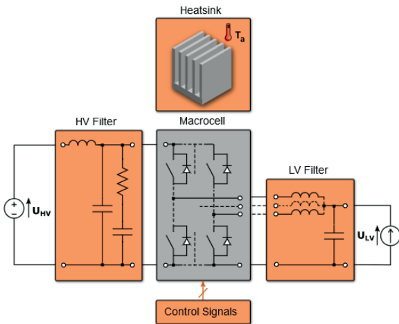
Fig. 8: Circuit of a multilevel non-isolated dc-dc converter
