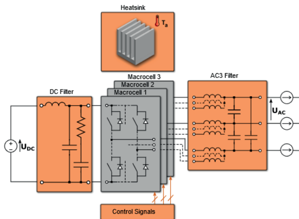
Fig. 9: Circuit of a multilevel three-phase inverter
