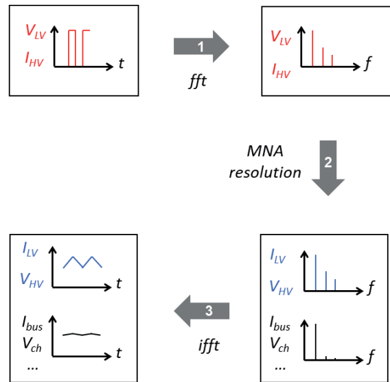
Fig. 3: Frequency resolution adapted to the commutation cell
