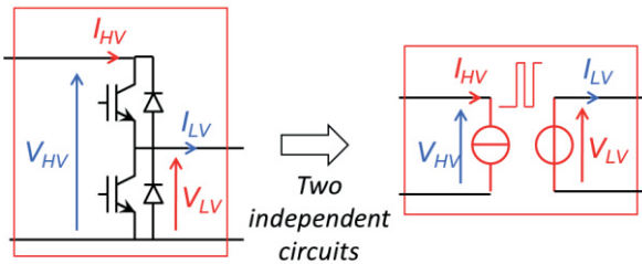
Fig. 1: Switching cell model
