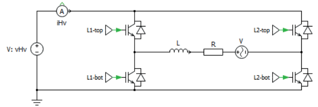
Fig. 5: Considered circuit composed of an inverter leg
