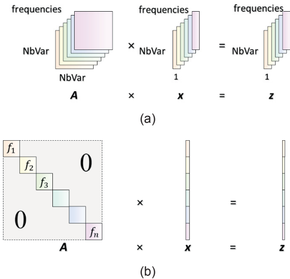
Fig. 4: MNA Matrix system built for all considered frequency
