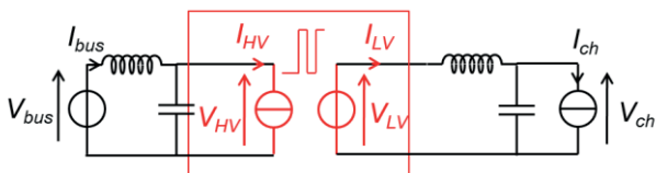
Fig. 2: Considered circuit with the commutation cell
