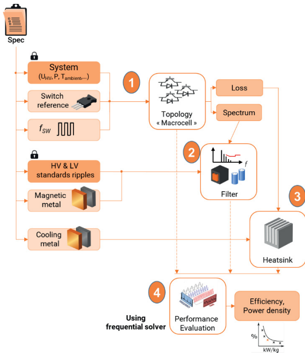
Fig. 10: Main steps of the design process
