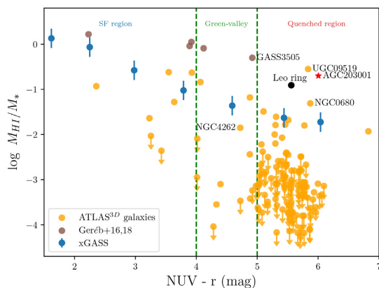
Figure 5. The H I gas fraction versus NUV - r plane. The blue points represent the median values from the xGASS survey (Catinella et al. 2018). AGC 203001 is marked with a red star and the Leo ring is marked with a black point. The yellow points represent the ATLAS 3D galaxies and the brown points represent the H I-excess galaxies (with GASS 3505 highlighted) from Geréb et al. (2016, 2018). The names of some of the H I-rich ATLAS 3D galaxies, UGC 09519 and NGC 0680, and a ring galaxy NGC 4262 are highlighted. The region within the green dashed line corresponds to the green-valley from Salim (2014), and the region on the left and right corresponds to the SF and quenched region, respectively. See text for discussion.
