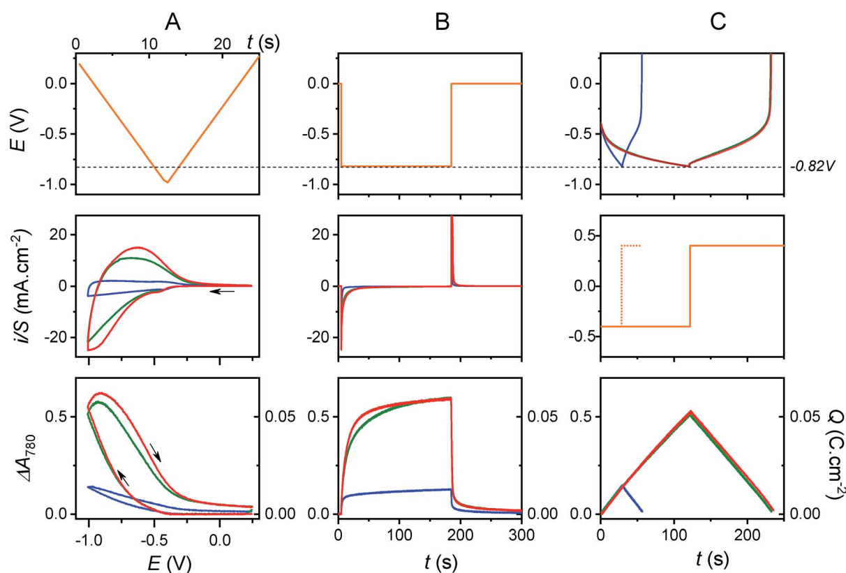
Fig. 2 Spectroelectrochemical characterization of a GLAD- \text{TiO}_2 / \text{TiO}_2 /ITO electrode in an aqueous electrolyte adjusted to pH 3.0 and containing (blue) 0.3 M KCl, (green) 0.25 M acetic acid and 0.3 M KCl, or (red) 0.25 M \text{AlCl}_3 . The orange lines in the top graphs in A and B and the middle graph in C represent the ramps or steps of potential or current which were applied during (A) the cyclic voltammetric, (B) chronoamperometric, and (C) galvanostatic ( 0.4 \text{ mA cm}^{-2} ) experiments. The current density is normalized to the geometric area ( S ) of the GLAD- \text{TiO}_2 electrode. The charge density Q is directly calculated from the visible absorbance change of the electrode at 780 nm and normalized to the geometric electrode area (see Materials and methods). The CVs/CVAs were performed at a scan rate \nu of 0.1 \text{ V s}^{-1} , while the chronoabsorptometric and galvanostatic experiments were carried out at a constant applied potential of E = -0.82 V or a constant applied current of j = 0.4 \text{ mA cm}^{-2} . All experiments were performed at 25^\circ \text{C} and potentials were quoted against the Ag/AgCl, sat. KCl reference electrode.
