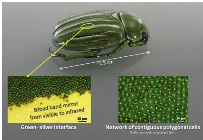
Fig. 2 Chrysin gloriosa , from a macroscopic view to micro-textures as observed in the green and silver bands.
