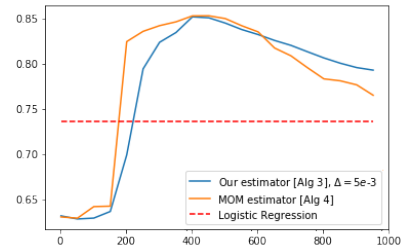
(e) N = 1000 , with 100 outliers
