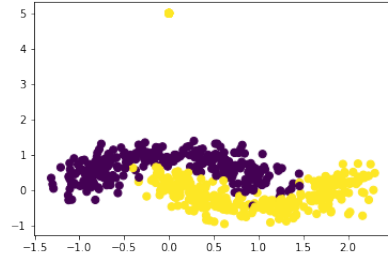
(a) “Two moons” dataset [39] with outliers.
