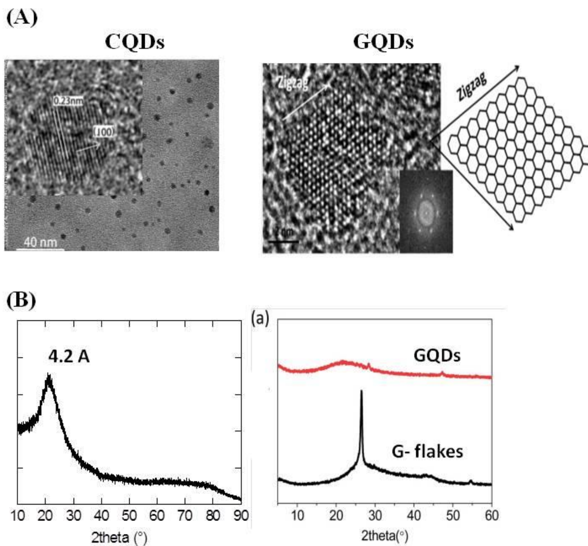
Figure 6: Transmission electron microscopy (TEM) and X-ray diffraction (XRD) examples: (A) TEM images of CQDs formed using ribonuclease A as a biomolecular templating agent under microwave irradiation (reprint with permission of Ref. 67 ) and GQDs synthesized using pristine few-layer graphene flakes as a precursor (reprint with permission of Ref. 66 ); (B) XRD patterns of CQDs (hydrothermal decomposition of 4-aminophenylboronic acid) 40 and GQDs (reprint with permission of Ref. 66 )
