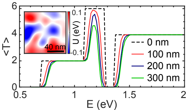
FIG. 5. Main panel: Average transmission coefficient as a function of the energy and for different L in the case of a \text{SiO}_2 substrate. The averaging is performed over 100 disorder realizations. Inset: Example of long-range potential profile realization for a \text{SiO}_2 substrate.
